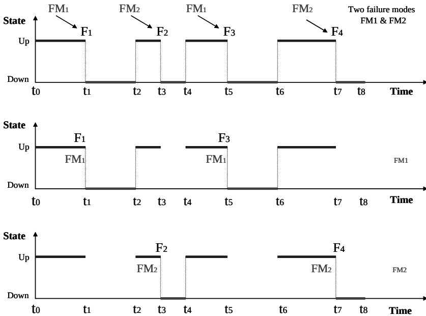
Figure 15.2. Representation of item states disaggregating per failure mode
