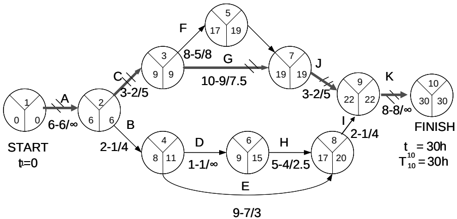
Figure 14.11. Maintenance project of the reactor repair using CPM—AOA. Normal times
