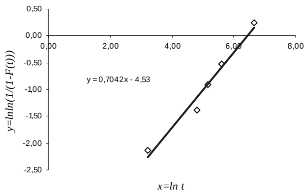
Figure 4.9. Points fit for coordinates change with t'=t-75
