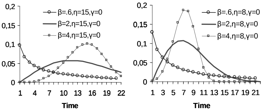
Figure 4.3. Sample Weibull functions with different parameters values
