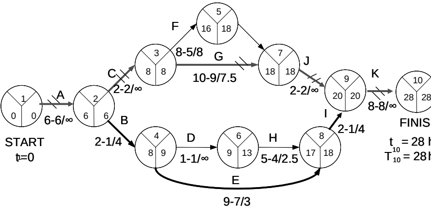
Figure 14. 14. New graph after the second iteration
