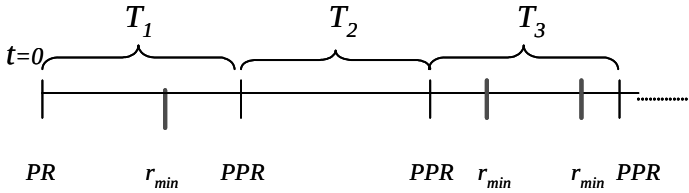
Figure 6.5. Equipment maintenance with PPR and minimal repairs option
