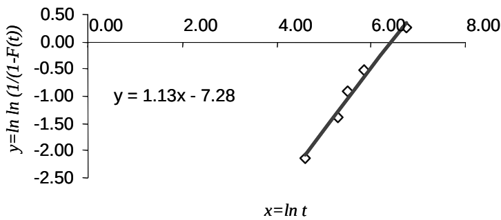
Figure 4.6. Straight line fitting points in Table 4.8
