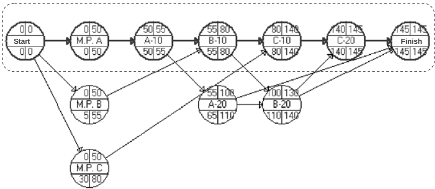
Figure 14.5. Maintenance project CPM—AON solution graph provided by WinQsb [3]
