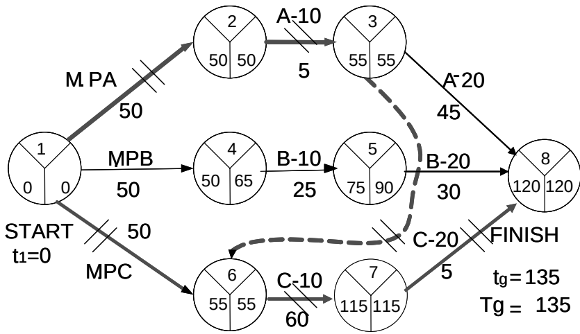
Figure 14.9. Maintenance project CPM—AOA graph with two resources V and 3 W
