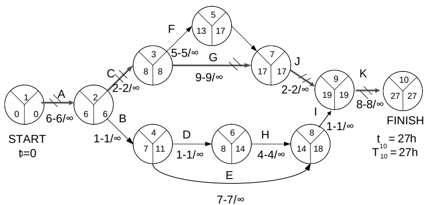
Figure 14.12. Maintenance project of the reactor repair using CPM—AOA. Crash times
