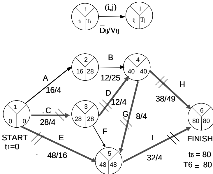
Figure 14.3. Sample PERT AOA network
