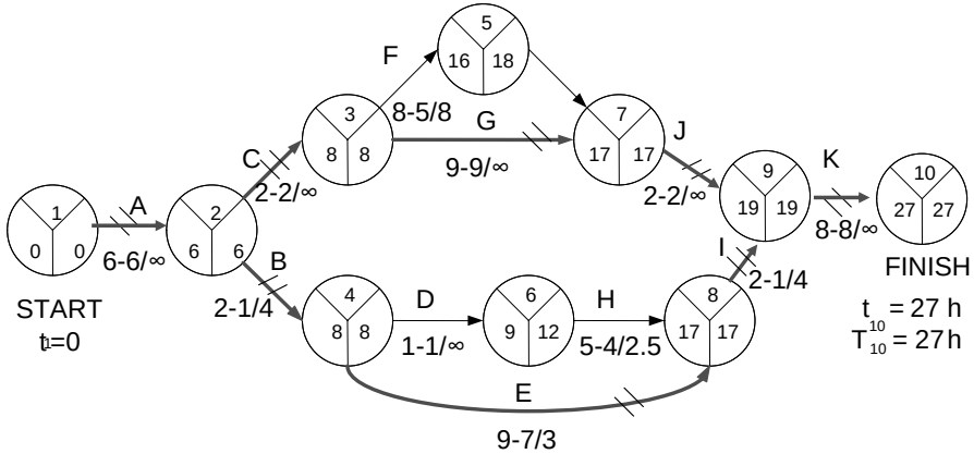
Figure 14.15. New graph after the third and final iteration
