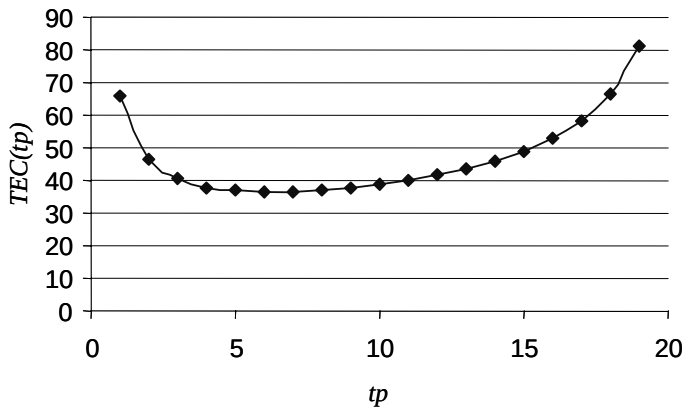
Figure 6.2. TEC(t_p) plot to find the optimum t_p value
