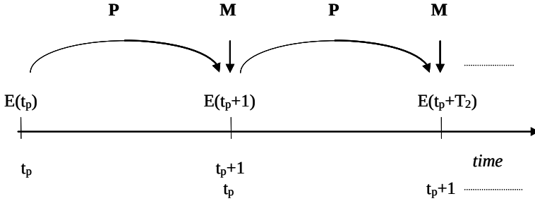
Figure 13.5. Limit cycle for straps with age based preventive maintenance
