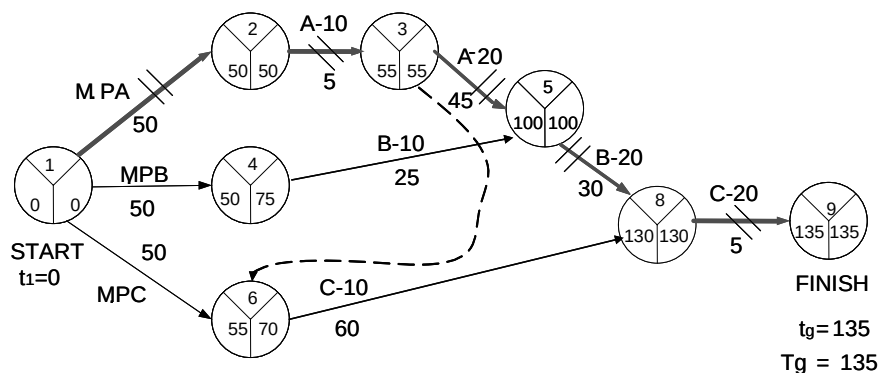
Figure 14.8. Maintenance project CPM—AOA graph with two resources V and one resource W
