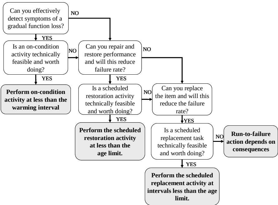
Figure 11.8. RCM logic
