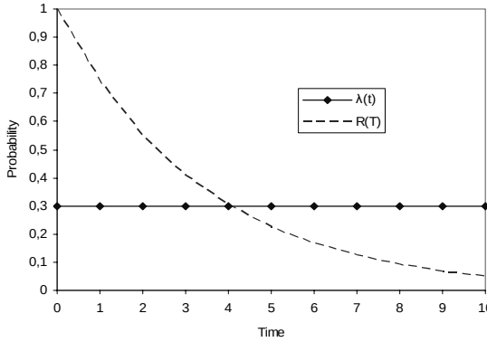
Figure 4.2. Reliability R(t) and failure rate \lambda(t) , when \lambda(t) is constant
