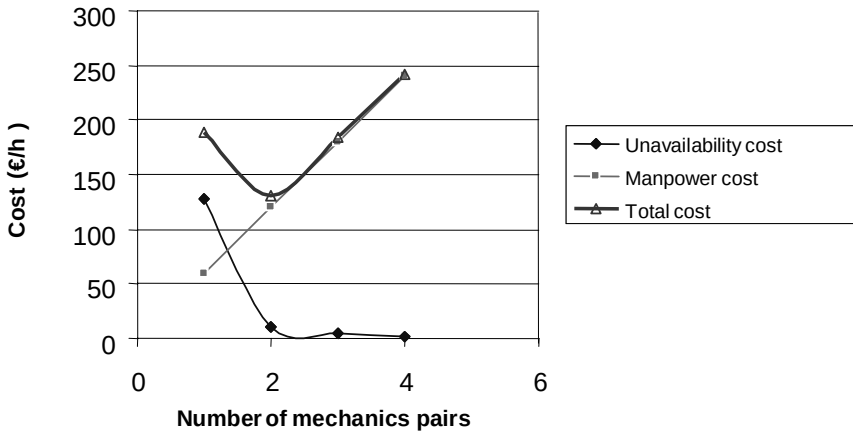
Figure 12.3. Total fleet cost as a function of the number of mechanics pairs
