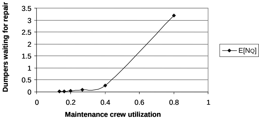
Figure 12.4. Maintenance crew utilization vs number of dumpers unavailable in the queue
