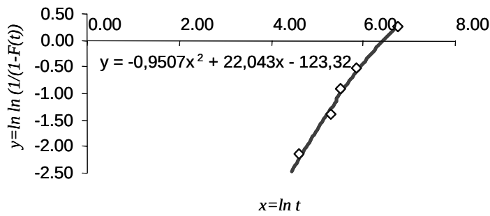
Figure 4.7. Curve (quadratic) line fitting points in Table 4.8
