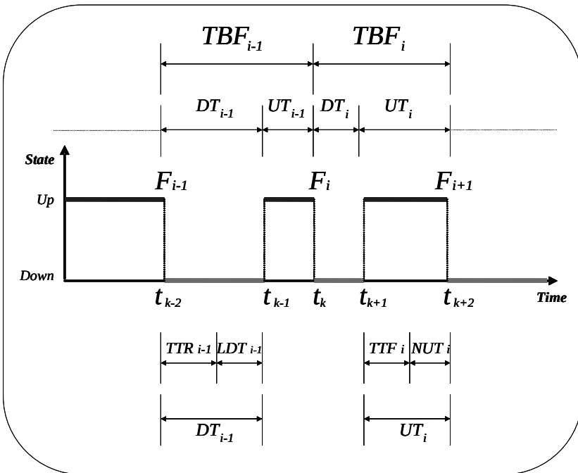
Figure 15.1. Representation of different times and states of an item subjected to failures
