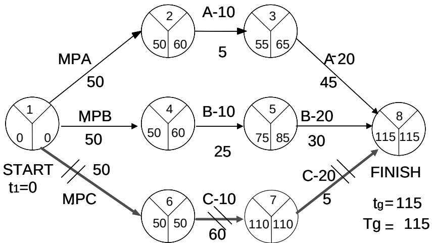
Figure 14.10. Maintenance project CPM—AOA graph with three resources V and 3 W
