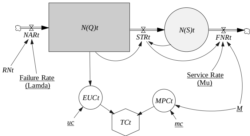
Figure 12.5. Stock and flow diagram of the dumpers maintenance problem
