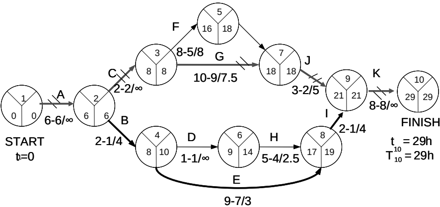
Figure 14. 13. New graph after the first iteration
