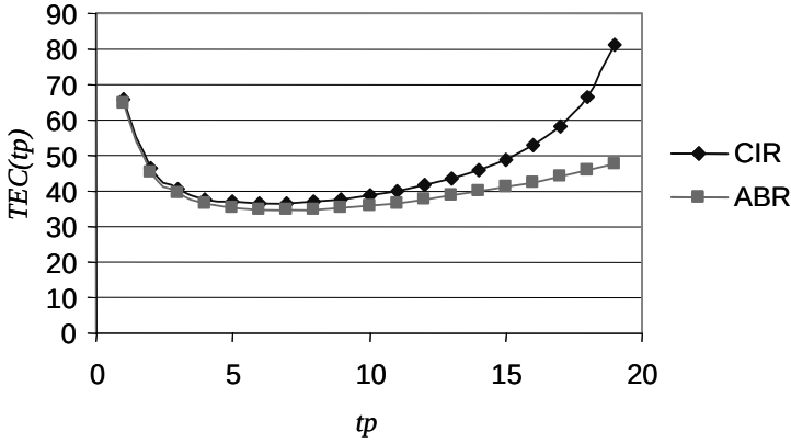
Figure 6.4. TEC(t_p) plot for CIR and ABR policies
