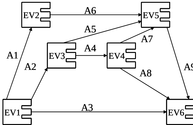
Figure 14.2. Sample CPM network (AOA)
