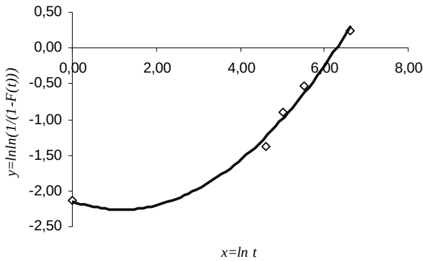
Figure 4.8. Points fit for coordinates change with t' = t - 100
