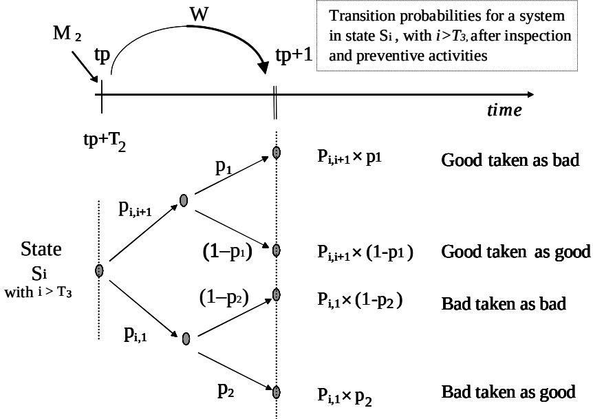
Figure 13.7. System update in the first transition after maintenance
