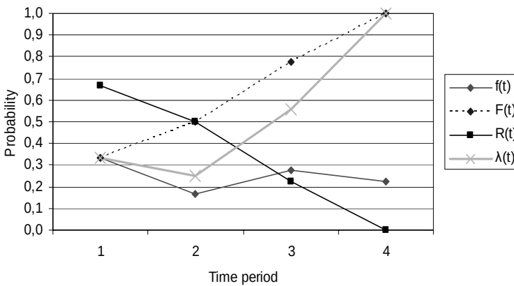
Figure 4.1. Graphical representation of basic functions
