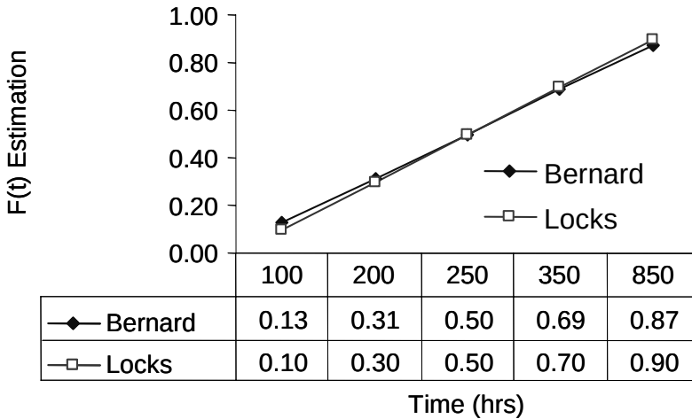
Figure 4.4. F(t) estimation using Bernard and Locks formulation
