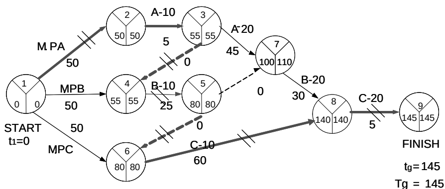
Figure 14.7. Maintenance project CPM—AOA graph
