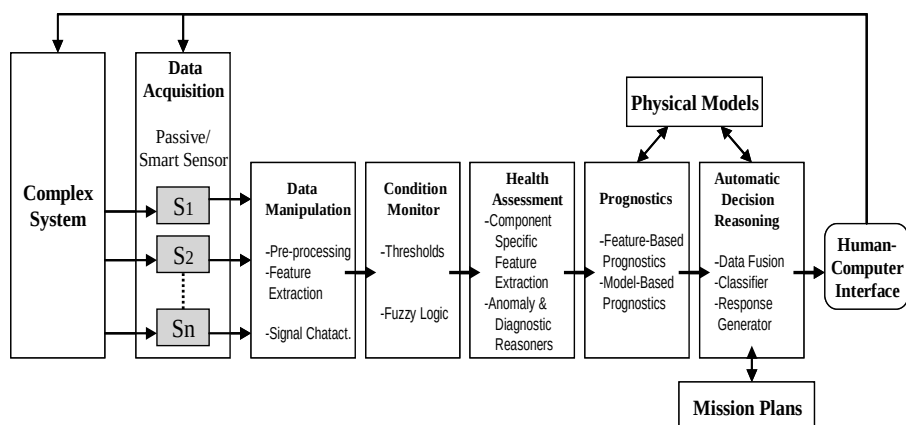
Figure 18.4. OSA-CBM architecture [35]
