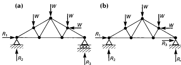
Fig. A3.1 The framework (a) is statically determinate. Framework (b) is statically indeterminate because the four external reactions cannot be solved from the three equations of equilibrium which can be derived.
