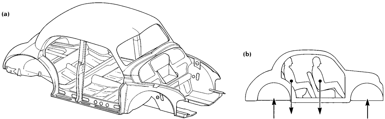
Fig. 4.15 The metal body of a motor car is an 'improved' non-form-active beam which spans between the road wheels.
