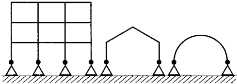
Fig. 5.3 Continuous structures. All are self-bracing and statically indeterminate.
