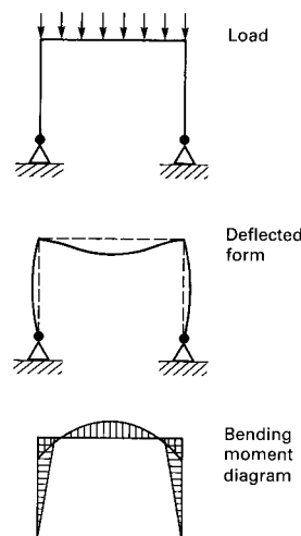
Fig. A3.7 A frame with rigid beam-to-column joints is statically indeterminate. The bending moment in the beam is less than it would be if hinge connections were provided, but at a cost of introducing bending moment into the columns.
