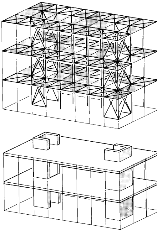
Fig. 2.11 A typical bracing scheme for a multi-storey framework. Vertical-plane bracing is provided in a limited number of bays and positioned symmetrically on plan. All other bays are linked to this by diagonal bracing in the horizontal plane at every storey level.
