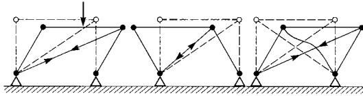
Fig. 2.8 Cross-bracing is used so that sway caused by instability is always resisted by a diagonal element acting in tension. The compressive diagonal buckles slightly and carries no load.
